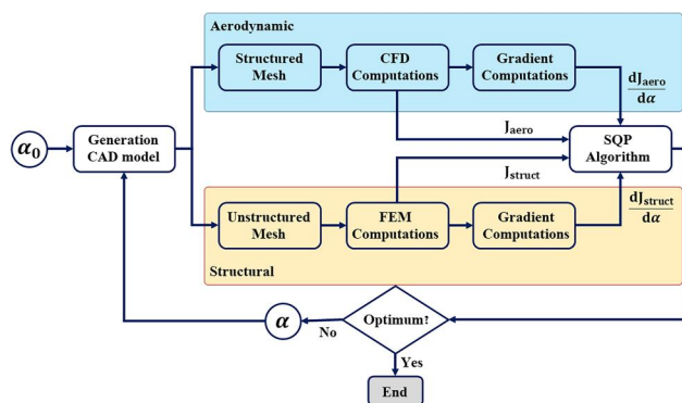
Fig. 4 Flow chart of aerodynamic-structural turbomachinery optimization algorithm
